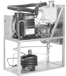
EF 800 Chassis
